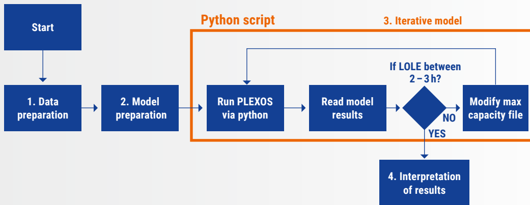
Figure 16 – Algorithm steps
