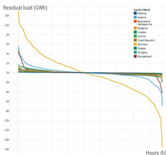
Figure 19 – Hourly residual load ramp of NSI East countries, in scenario National Trends 2030
