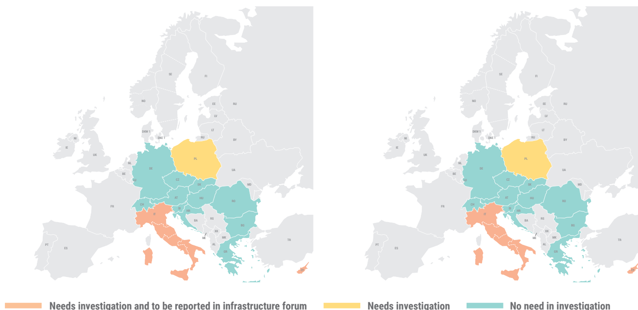
Figure 20 – Ratio of nominal transmission capacity (thermal capacity) to the peak load in 2030, in the case where Europe would stop all grid reinforcement after 2022 (left) and with the expected grid in 2025 (right)
