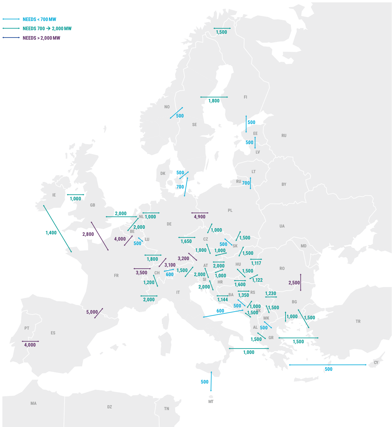
Figure 1.3 – Needs for capacity increases identified in the 2040 horizon, additional to the 2025 network (SEW based needs 2040)*.
