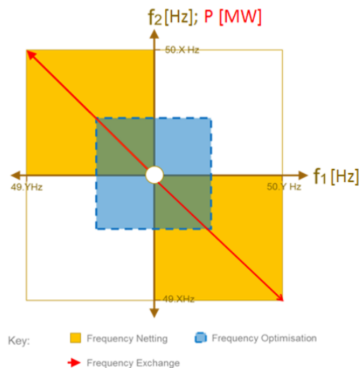
Figure 10: Illustration of the frequency netting and exchange
