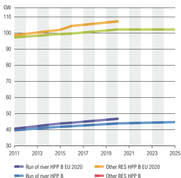
Figure 4.55: Comparison between Scenario B and Scenario EU 2020 for run of river HPP and other renewable HPP installed capacity, January 7 p.m.
