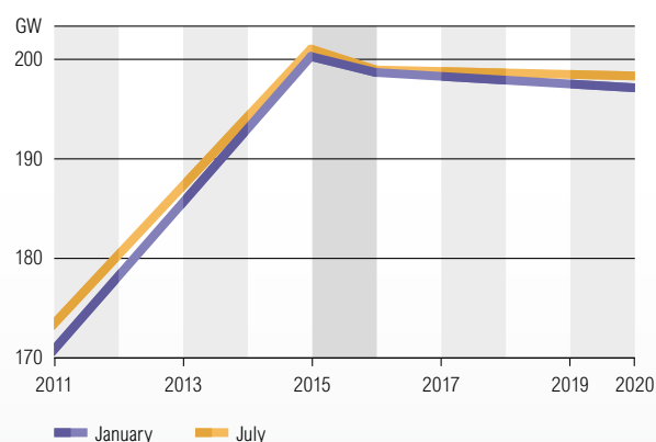
Figure 4.27: ENTSO-E gas generating capacity forecast, Scenario EU 2020
