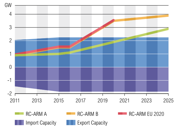
Figure 6.4: RC – ARM Comparison, Sc A, Sc B and Sc EU 2020, January 7 p.m.
