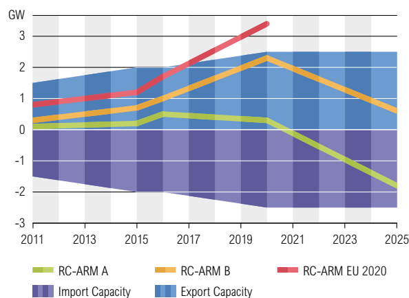
Figure 6.15: RC – ARM Comparison, Sc A, Sc B and Sc EU 2020, January 7 p.m.
