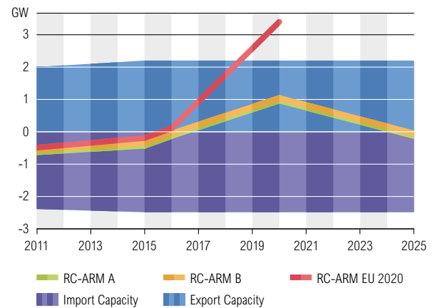
Figure 6.32: RC – ARM Comparison, Sc A, Sc B and Sc EU 2020, January 7 p.m.
