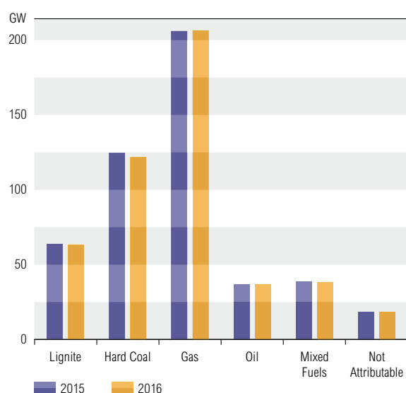
Figure 4.40: ENTSO-E fossil fuels generating capacity breakdown in 2015 and 2016, Scenario B
