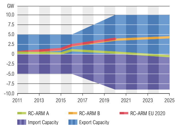
Figure 6.5: RC – ARM Comparison, Sc A, Sc B and Sc EU 2020, January 7 p.m.
