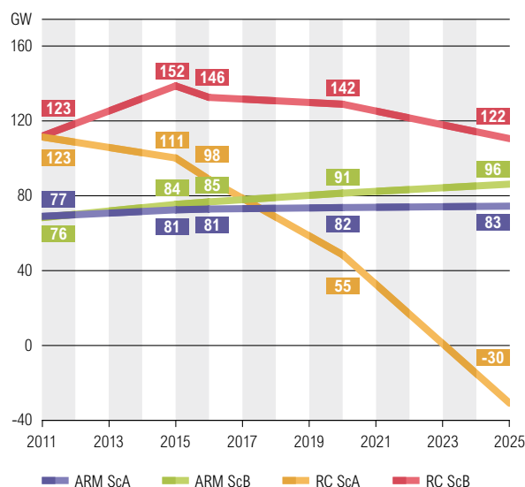
Figure 2.6: ENTSO-E RC and ARM comparison, Scenarios A & B, January 7 p.m.
