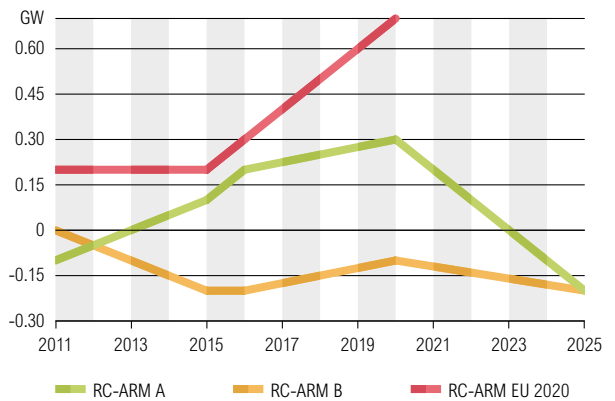
Figure 6.6: RC – ARM Comparison, Sc A, Sc B and Sc EU 2020, January 7 p.m.
