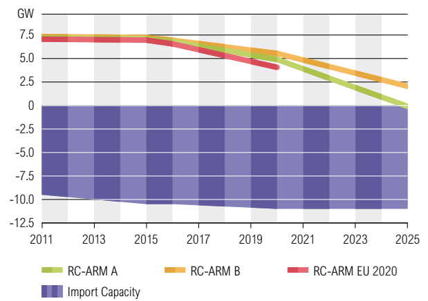
Figure 6.20: RC – ARM Comparison, Sc A, Sc B and Sc EU 2020, January 7 p.m.
