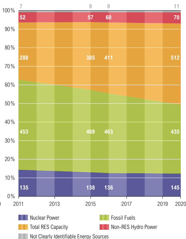
Figure 4.14: ENTSO-E total NGC mix, Scenario EU 2020, January 7 p.m., values in GW
