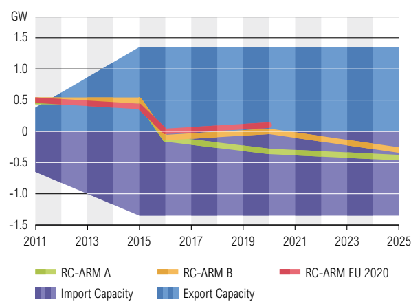
Figure 6.26: RC – ARM Comparison, Sc A, Sc B and Sc EU 2020, January 7 p.m.
