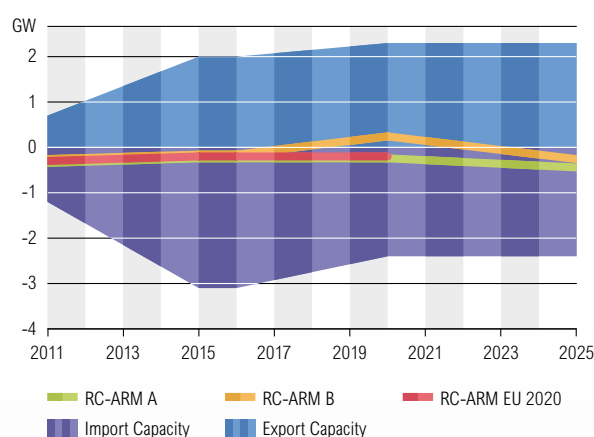
Figure 6.24: RC – ARM Comparison, Sc A, Sc B and Sc EU 2020, January 7 p.m.
