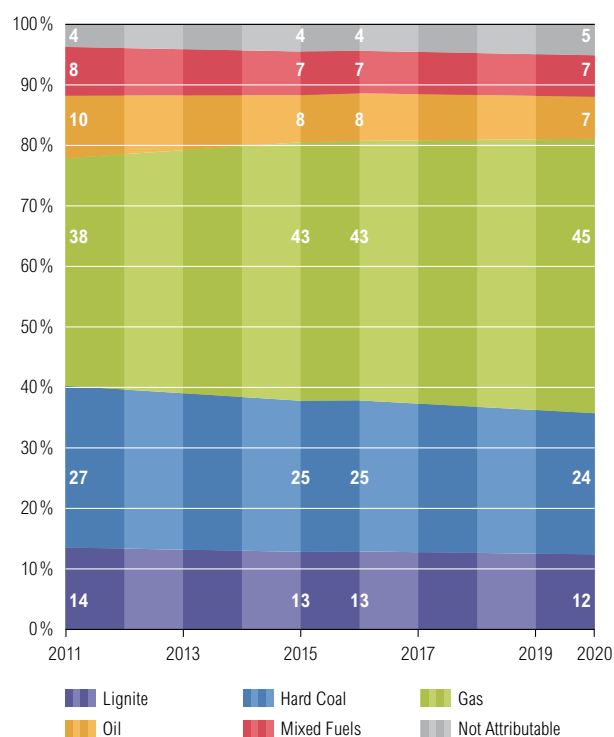
Figure 4.24: ENTSO-E fossil fuels generating capacity breakdown, Scenario EU 2020, January 7 p.m.
