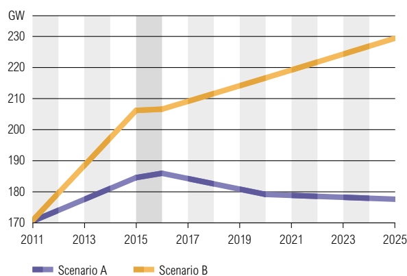
Figure 4.37: ENTSO-E gas generating capacity forecast, Scenarios A & B
