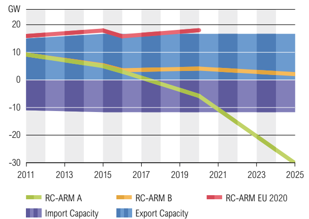
Figure 6.13: RC – ARM Comparison, Sc A, Sc B and Sc EU 2020, January 7 p.m.
