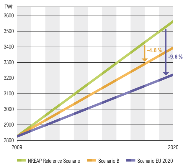
Figure 4.81: Impact of efficiency measures on electricity demand at EU level
