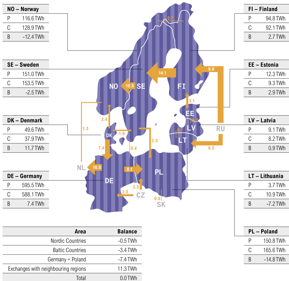
Figure 8.3: Energy balance and net flows for each country in RGS in 2015, a year with extremely low inflow
