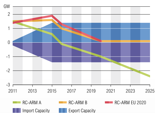
Figure 6.18: RC – ARM Comparison, Sc A, Sc B and Sc EU 2020, January 7 p.m.
