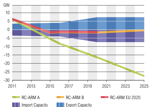
Figure 6.14: RC – ARM Comparison, Sc A, Sc B and Sc EU 2020, January 7 p.m.
