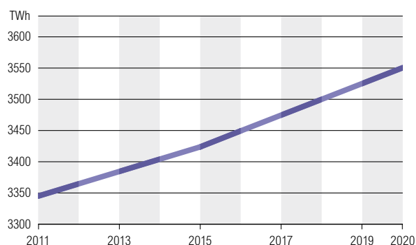
Figure 2.1: ENTSO-E consumption forecast for the Scenario EU 2020
