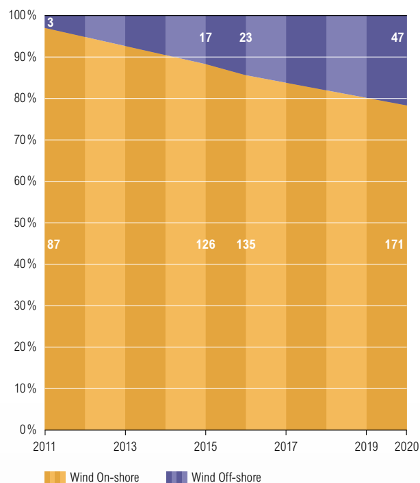
Figure 4.53: ENTSO-E total wind breakdown, January 7 p.m., Scenario EU 2020, values in GW
