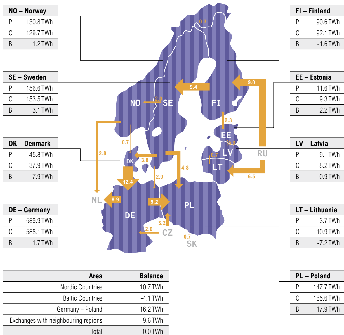
Figure 8.2: Energy balance and net flows for each country in RGBS in 2015, a year with low inflow
