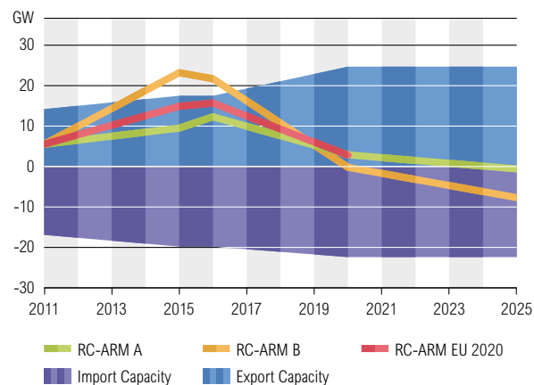
Figure 6.8: RC – ARM Comparison, Sc A, Sc B and Sc EU 2020, January 7 p.m.
