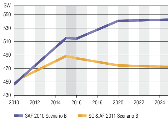
Figure 4.33: ENTSO-E Fossil fuels generating capacity forecast, comparison of Scenario B in SO & AF 2011 and SAF 2010
