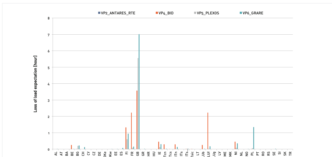
Figure 31 - LOLE 2020 Sensitivity II. (LOLE of CY= 16 h not shown for visibility since ENS is just 30 MW)
