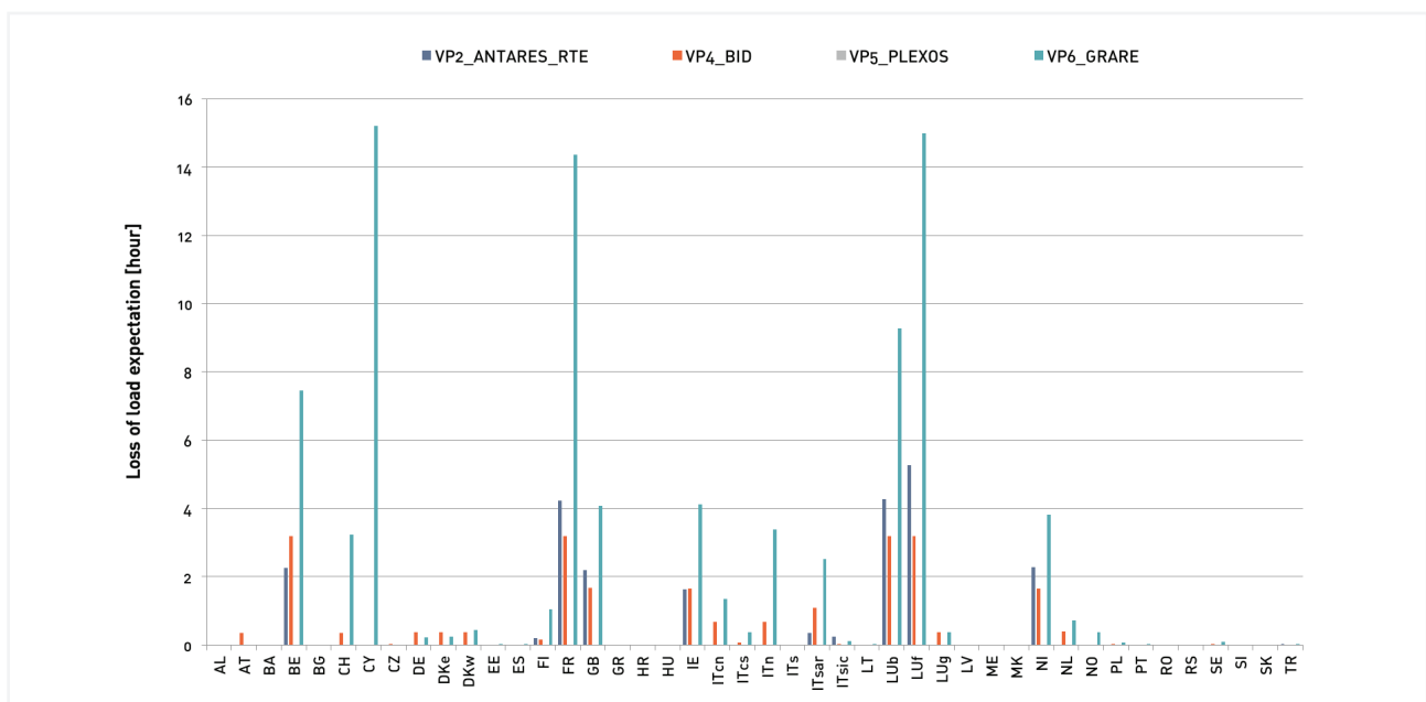
Figure 35 LOLE 2025 Sensitivity I
