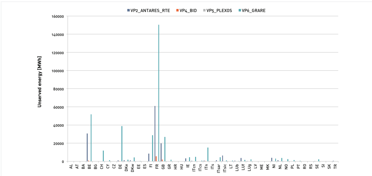
Figure 32 2025 ENS Base Case
