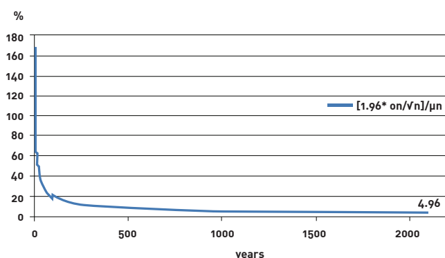
Figure 13 – Example of confidence interval reached by the simulations in MAF 2016
