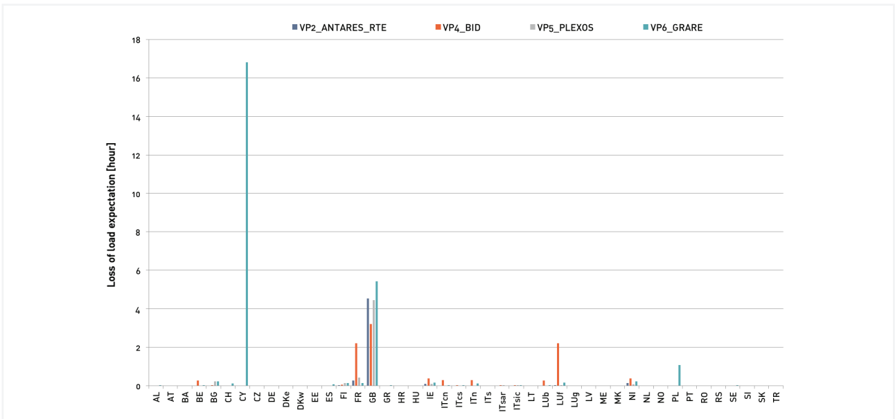
Figure 29 - LOLE 2020 Sensitivity I. (LOLE of CY= 16 h not shown for visibility since ENS is just 30 MW)
