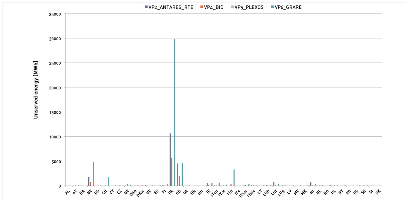
Figure 34 ENS 2025 Sensitivity I
