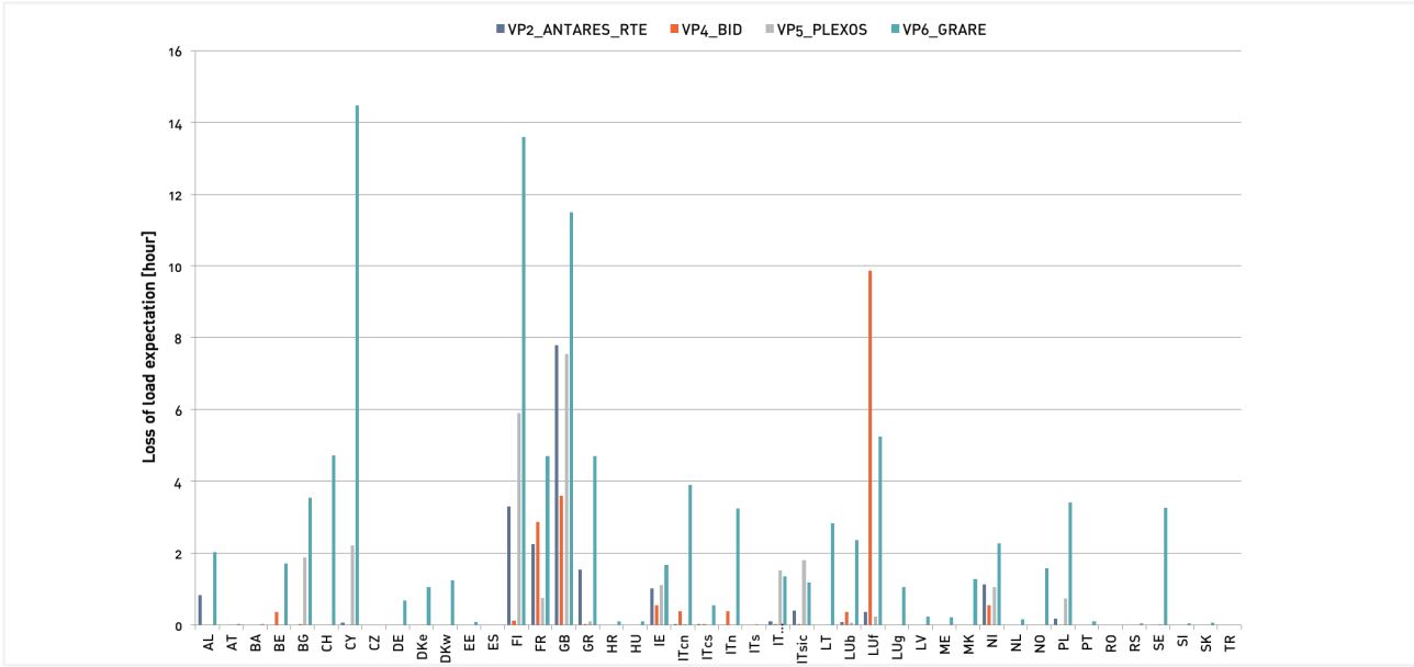
Figure 27 Loss of Load Expectation (LOLE) distribution (Base Case 2020)
