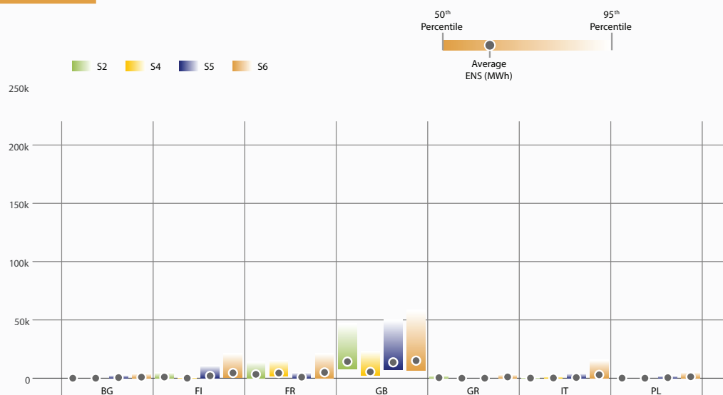
FIGURE 5 – ENS 2020 BASE CASE: P50, AVERAGE, P95 PERCENTILES. (ONLY FOR COUNTRIES FROM PREVIOUS MAP WITH ENS > 300 MWh)
