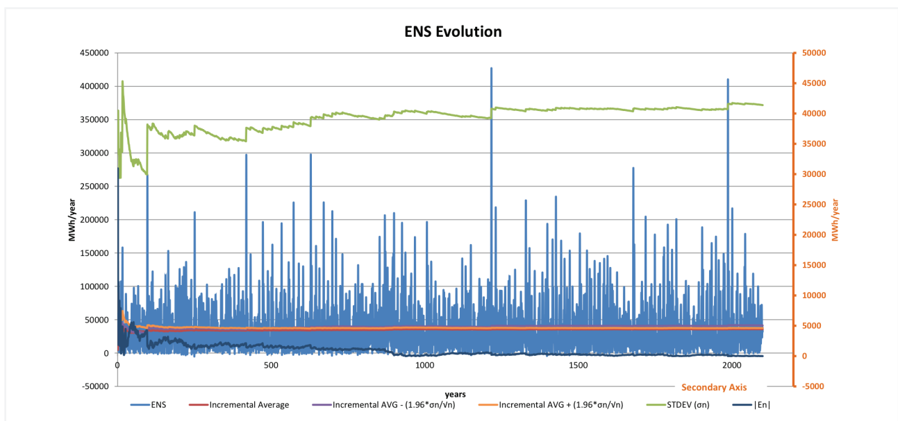
Figure 25 – Example of convergence on all the MC years (Base Case - VP6)
