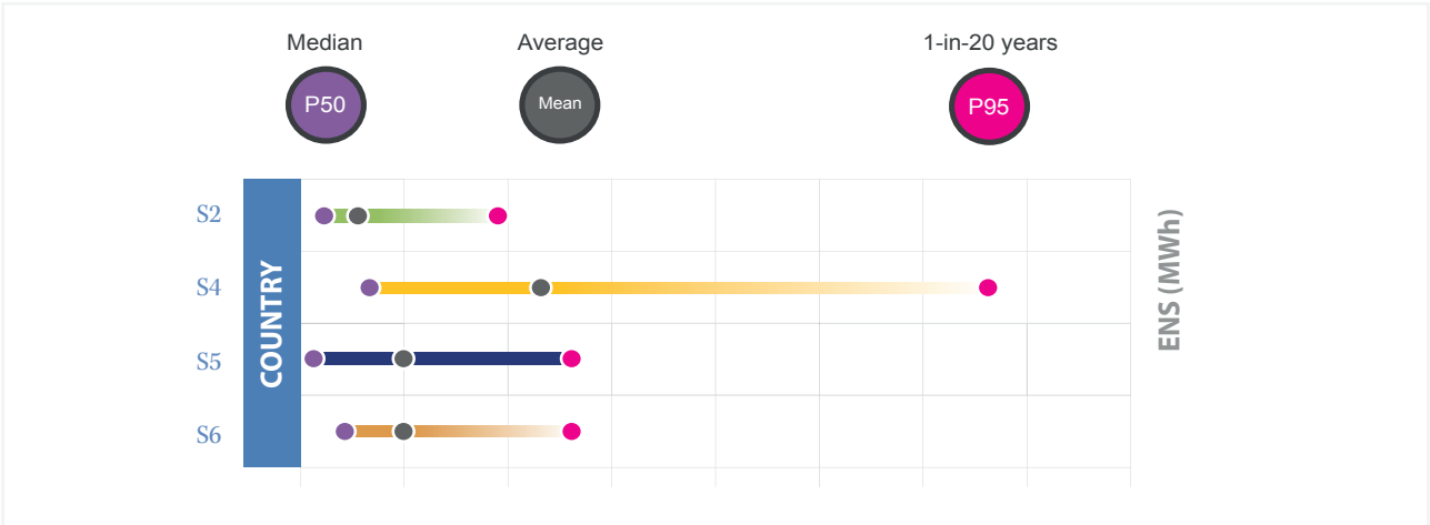
FIGURE 3 – EXPLANATORY EXAMPLE OF PRESENTATION OF MAIN RESULTS (P50, MEAN, P95) OBTAINED BY THE 4 MARKET MODELLING TOOLS USED (DENOTED BY THE DIFFERENT COLOR BARS).
