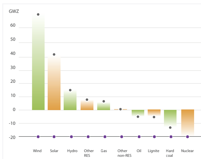
Figure 18 - Differences in Net Generating Capacity between 2025 and 2020, ENTSO-E level 11
