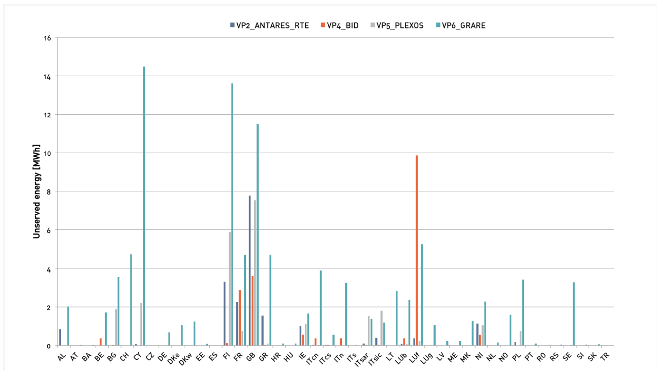
Figure 24 – Energy Non Served (ENS) distribution (Base case 2020)
