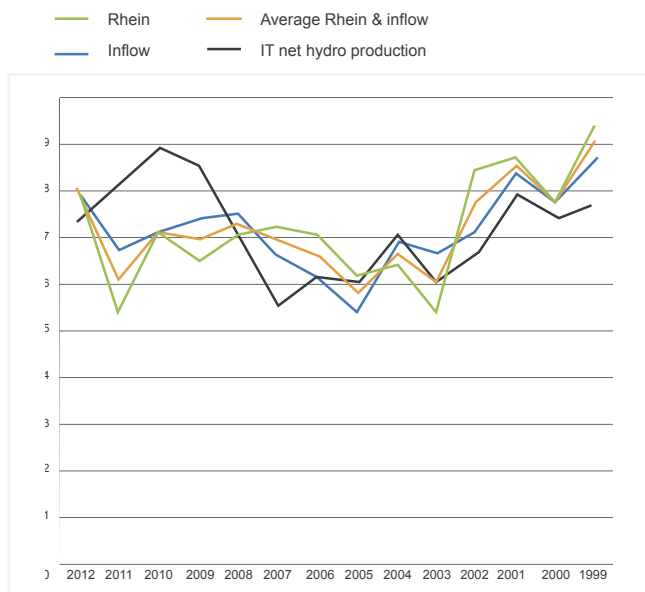
Figure 22 – Switzerland and Italy historical hydro production (Note that the years are reversed in the x-axis)
