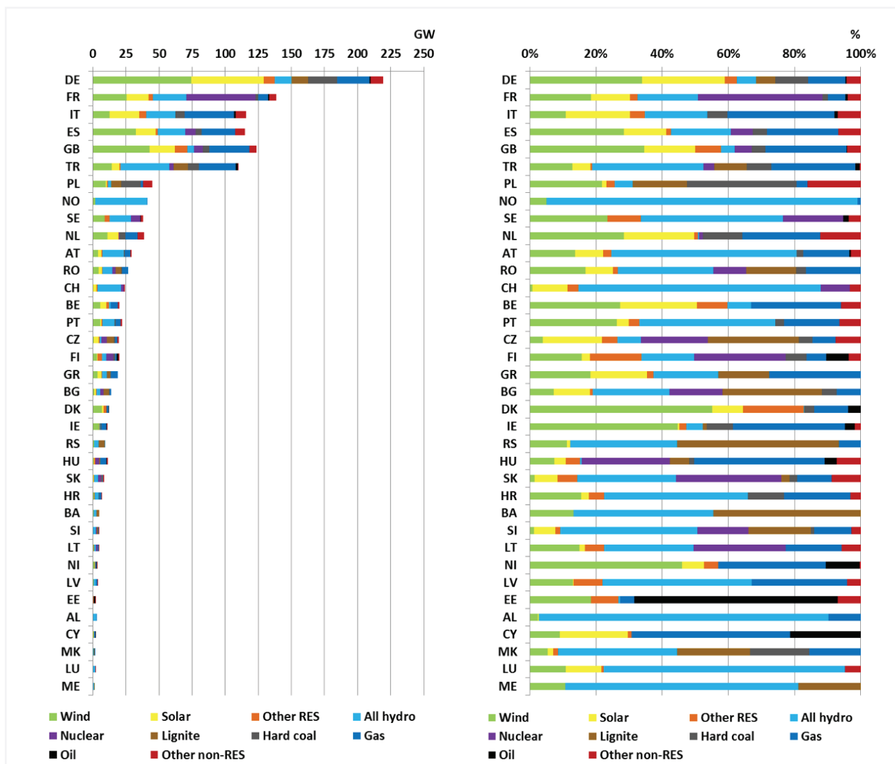
Figure 17 – Detailed Net Generating Capacity structure per country, year 2025
