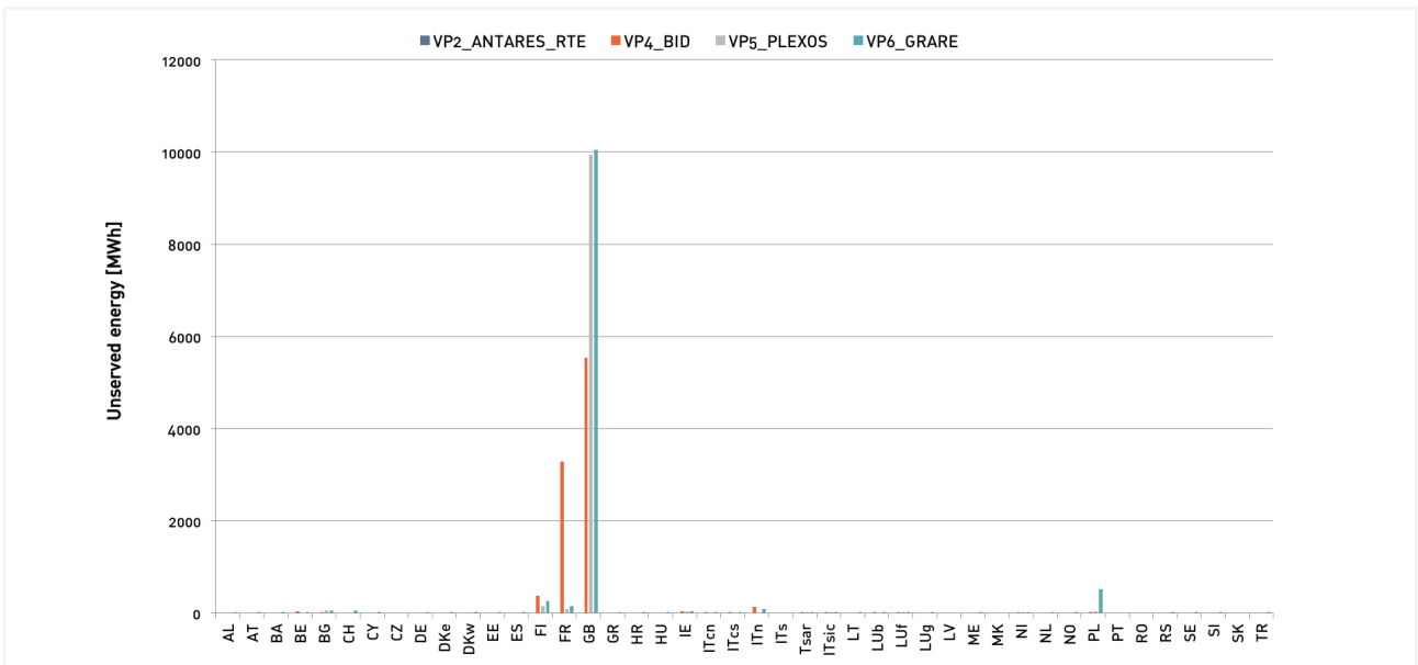
Figure 30 - ENS 2020 Sensitivity II
