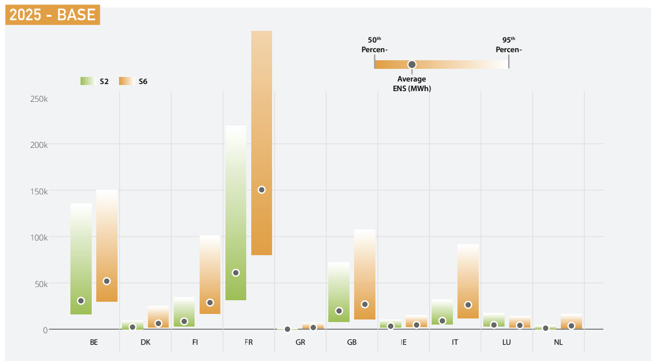
FIGURE 8 - 2025 ENS BASE CASE - P50, AVERAGE, P95 PERCENTILES. (NOTE: ONLY FOR COUNTRIES IN RED IN THE 2025 COLUMN OF THE 'OVERVIEW TABLE' - FOR FURTHER DETAILS SEE CHAPTER 5 )
