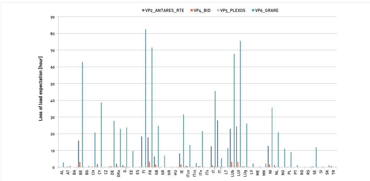
Figure 33 2025 LOLE Base Case
