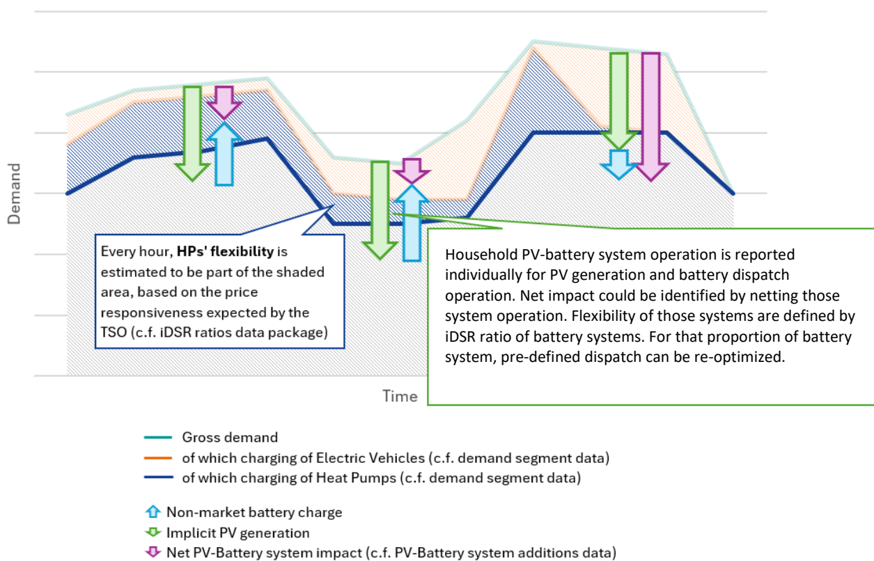
Figure 4 | Implicit DSR
