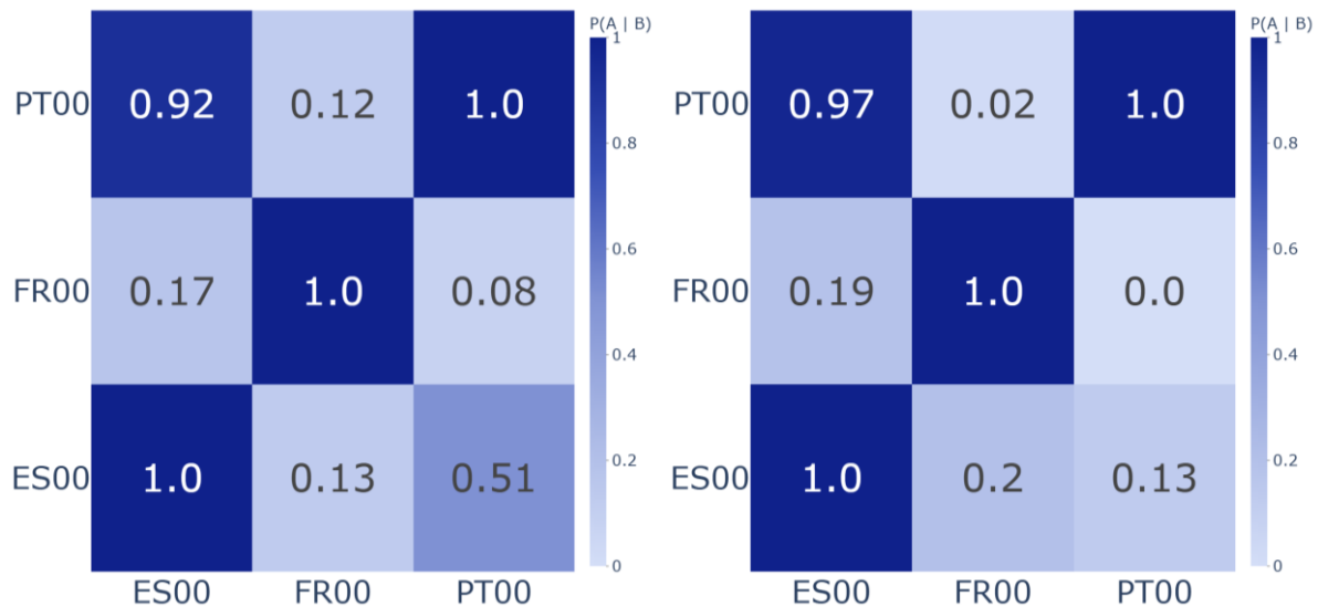
Figure 25: Boundaries of simultaneous scarcity events in South-West Europe for the central reference scenario of risk aversion modelling in TY 2028
