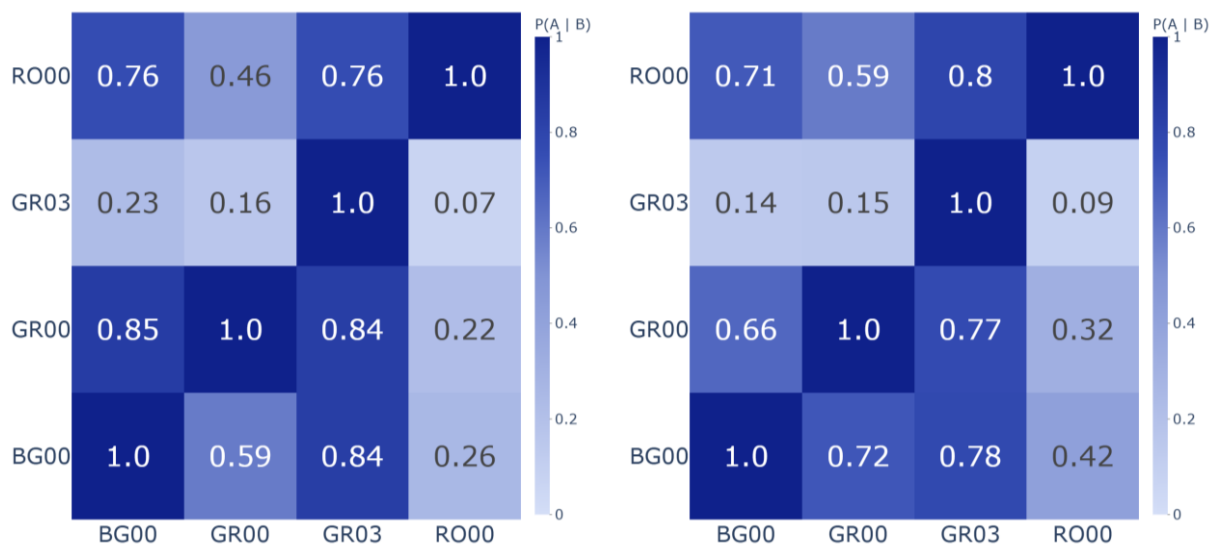
Figure 23: Boundaries of simultaneous scarcity events in South-East Europe for the central reference scenario of risk aversion modelling in TY 2033
