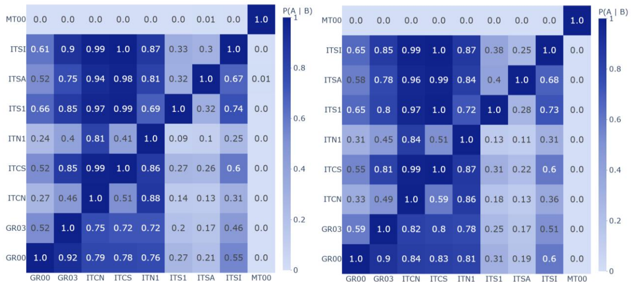
Figure 10: Boundaries of simultaneous scarcity events in Greece – Italy for the central reference scenario of risk aversion modelling in TY 2030
