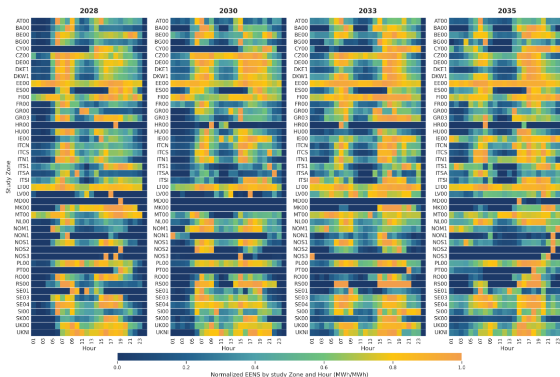
Figure 30: Boundaries of scarcity temporal distribution in study zones and hour for the central reference scenario of risk aversion modelling
