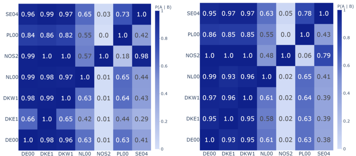
Figure 14: Boundaries of simultaneous scarcity events in Hansa for the central reference scenario of risk aversion modelling in TY 2030
