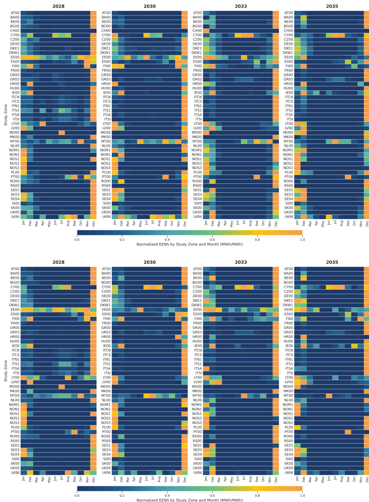
Figure 31: Boundaries of scarcity temporal distribution in study zones and year-month for the central reference scenario of risk aversion modelling
