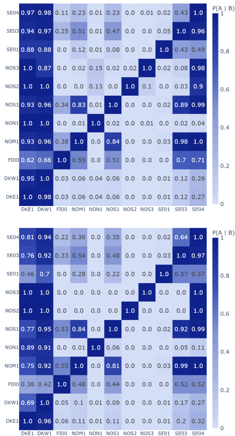
Figure 20: Boundaries of simultaneous scarcity events in the Nordic region for the central reference scenario of risk aversion modelling in TY 2035
