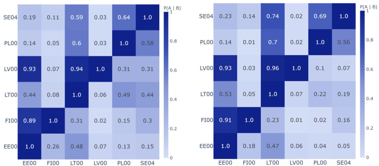
Figure 3: Boundaries of simultaneous scarcity events in the Baltics for the central reference scenario of risk aversion modelling in TY 2033
