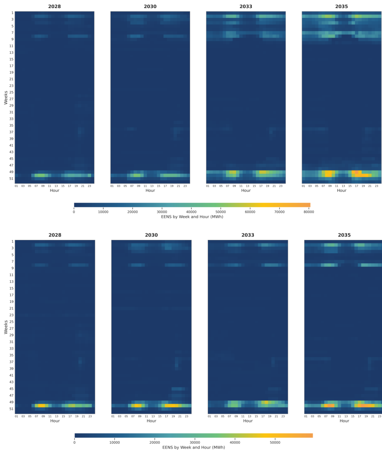
Figure 29: Boundaries of Scarcity temporal distribution in Year-week and hour of central reference scenario on risk aversion modelling
