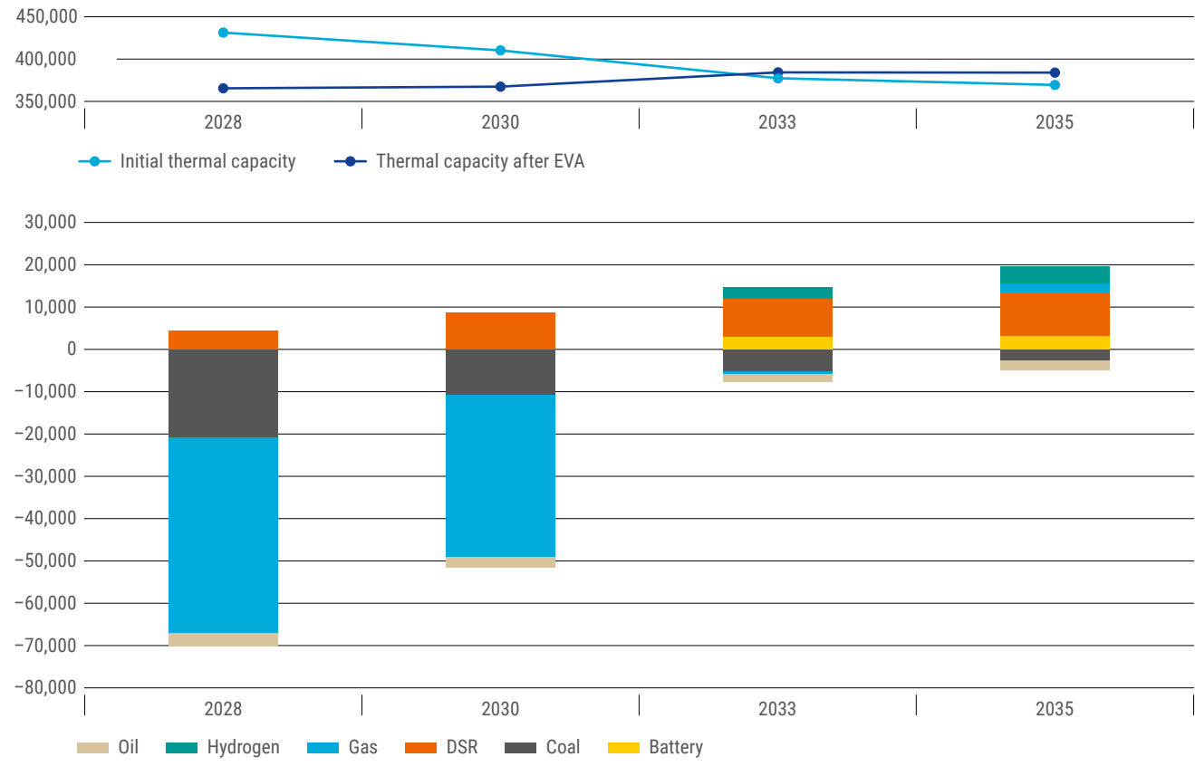
Figure 1: Net effect of the EVA on the European mix
