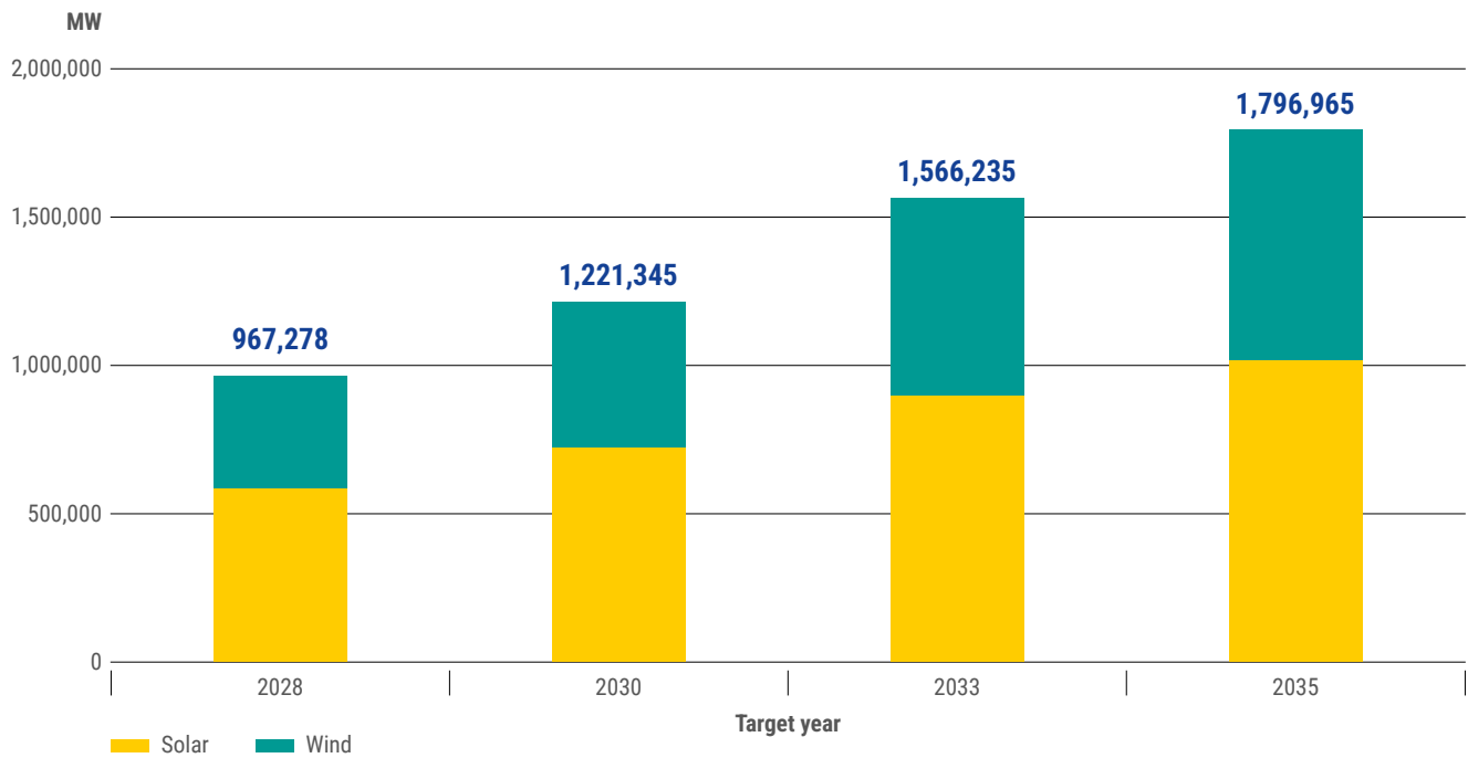
Figure 2: Anticipated wind and solar capacity evolution [MW]
