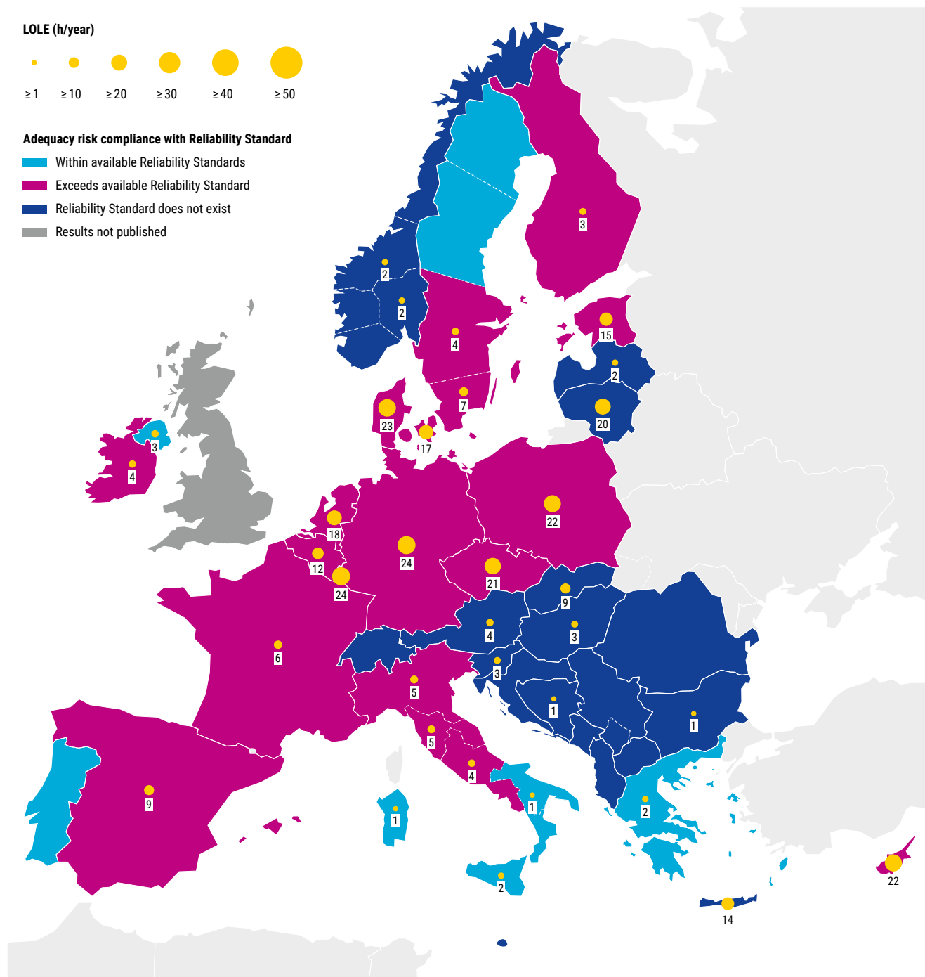
Figure 9: LOLE values in 2035 (mainly LOLE and EENS)
