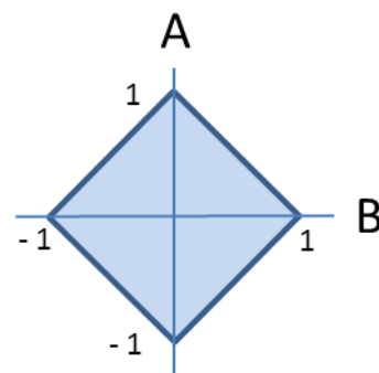
Figure 6: Two-dimensional projection of cube-shaped domain for C = 0
