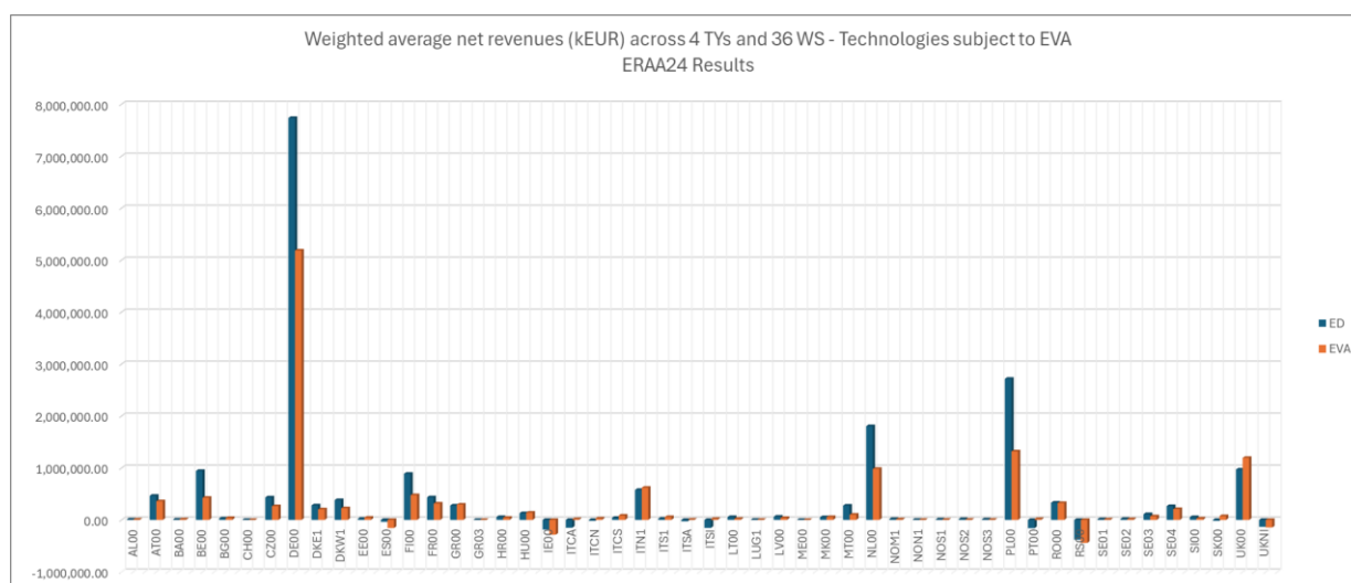
Figure 19: Weighted average net revenues (kEUR) per study zone – ERAA 2024 results
