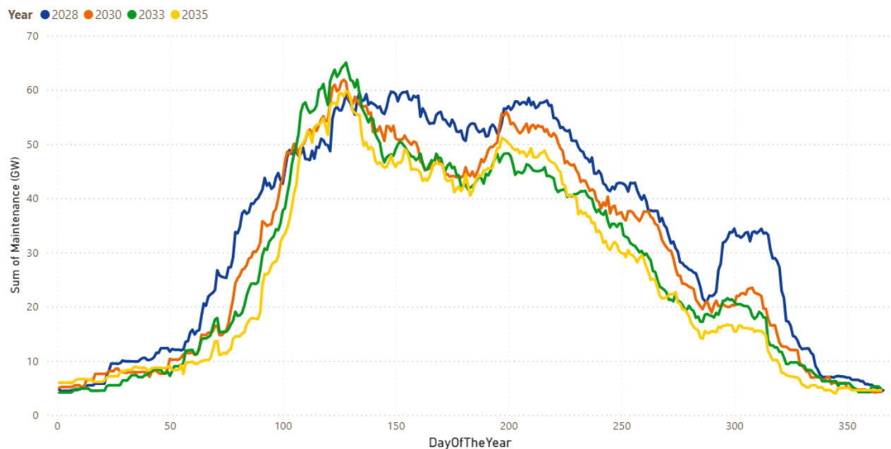
Figure 6: Pan-EU thermal capacity in maintenance
