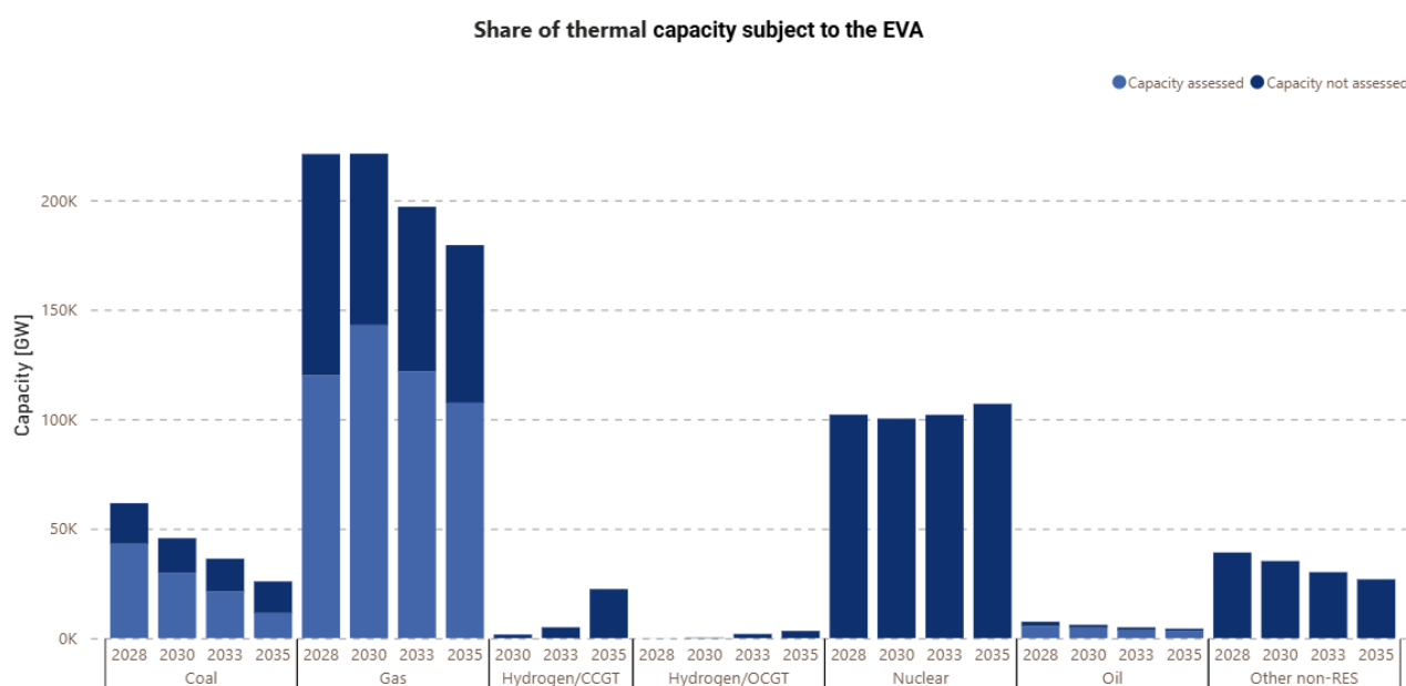
Figure 10: Share of thermal capacity subject to the EVA
