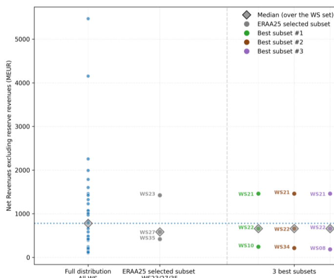
Figure 2: Post-EVA revenue distribution (TY and study zone's average) for the hurdle-premium only approach
