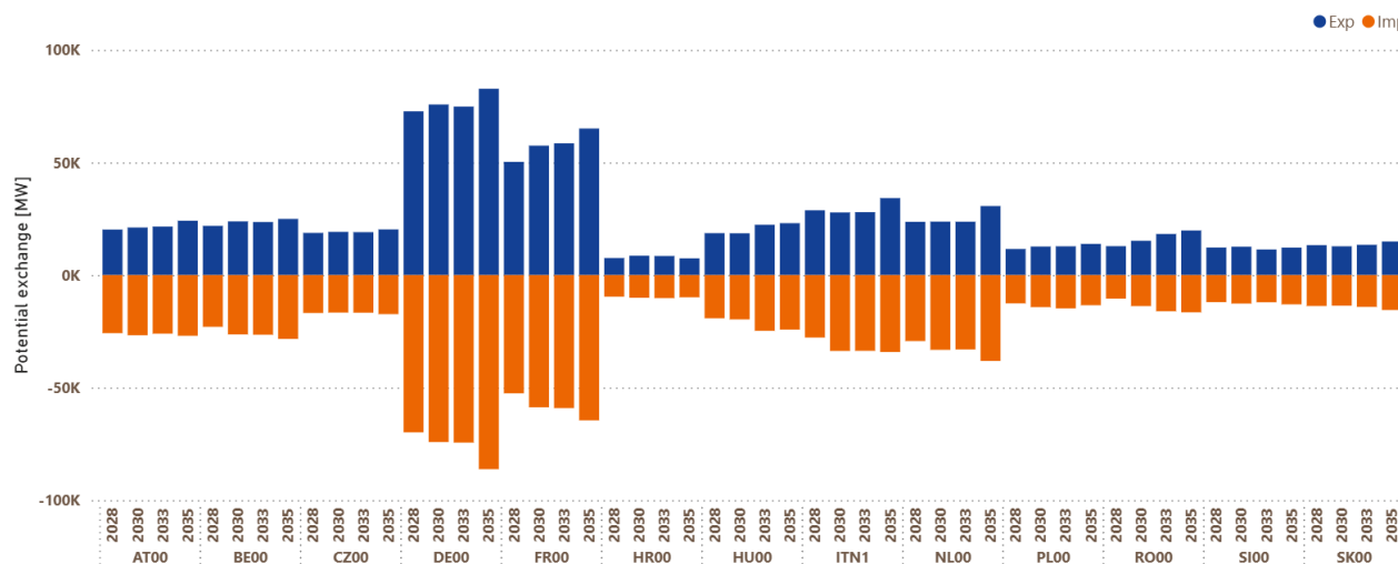
Figure 8: Illustrative theoretical maximum export and import capacities for all TYs 6
