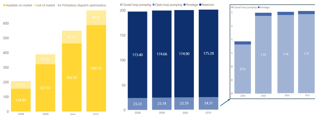
Figure 4: Battery storage capacity [GWh], hydro storage capacity [TWh]
