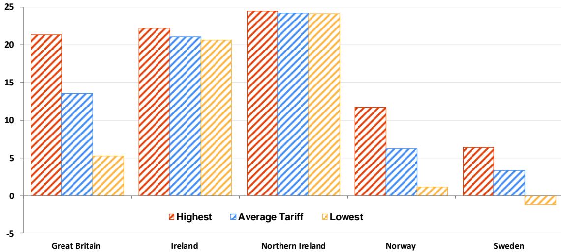
Chart 7.5. Impact of location on the Unit Transmission Tariffs (€/MWh)
