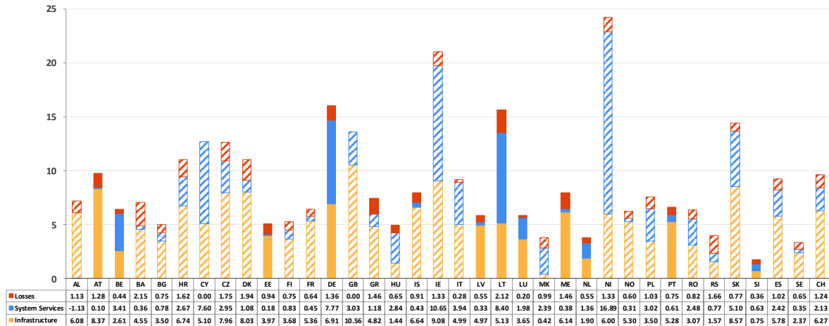
Chart 7.6. Components of TSO costs of the Unit Transmission Tariffs (€/MWh)
