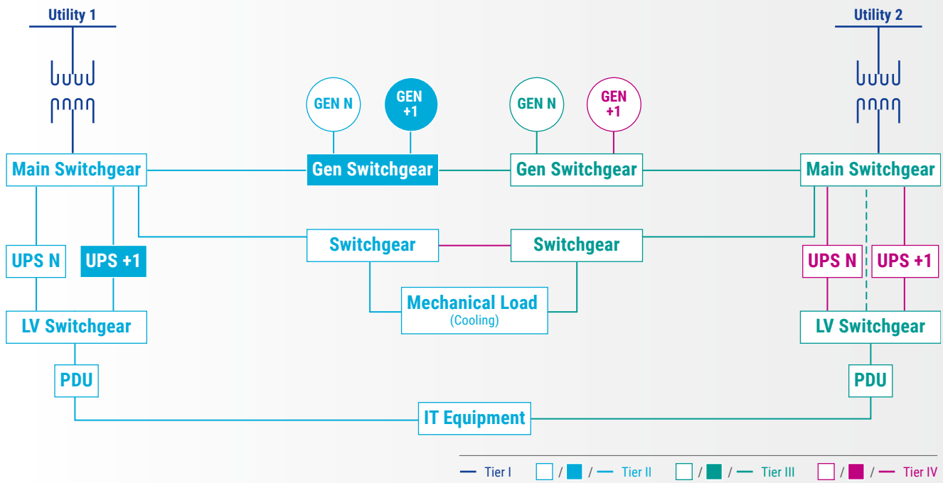
Figure 5: Illustrative power architectures by tier (redundancy level)
