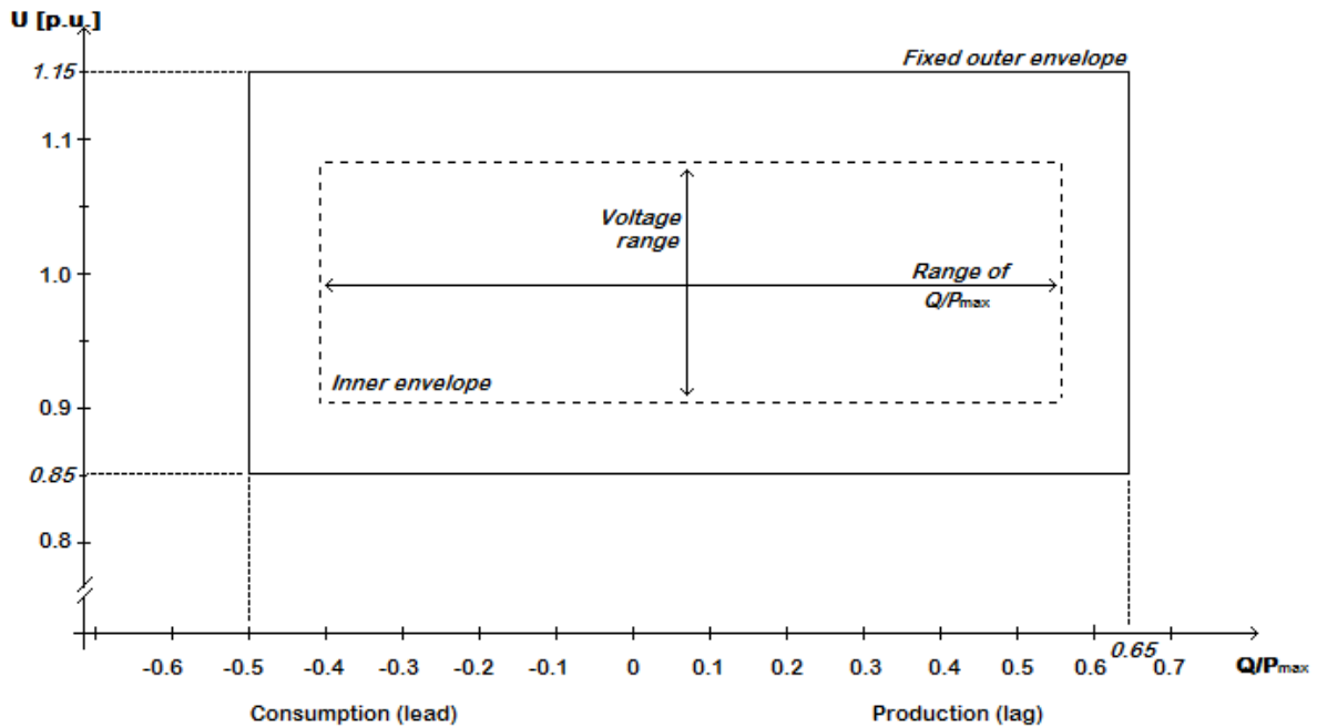
Figure 5: The diagram represents boundaries of a U-Q/Pmax-profile with U being the voltage at the connection points expressed by the ratio of its actual value to its reference 1 pu value in per unit, and Q/Pmax the ratio of the reactive power to the maximum HVDC active power transmission capacity. The position, size and shape of the inner envelope are indicative and shapes other than rectangular may be used within the inner envelope. For profile shapes other than rectangular, the voltage range represents the highest and lowest voltage points in this shape. Such a profile would not give rise to the full reactive power range being available across the range of steady-state voltages.
