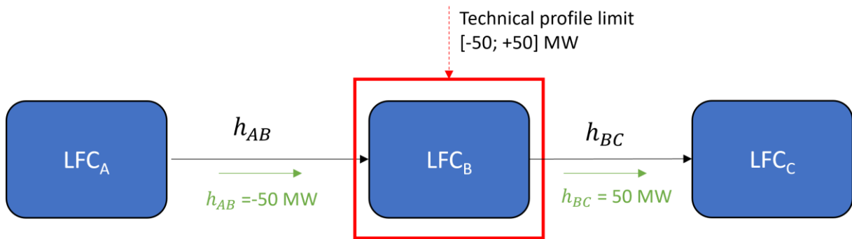
Figure 13: Example of a saturation of a border in case of technical profiles.
