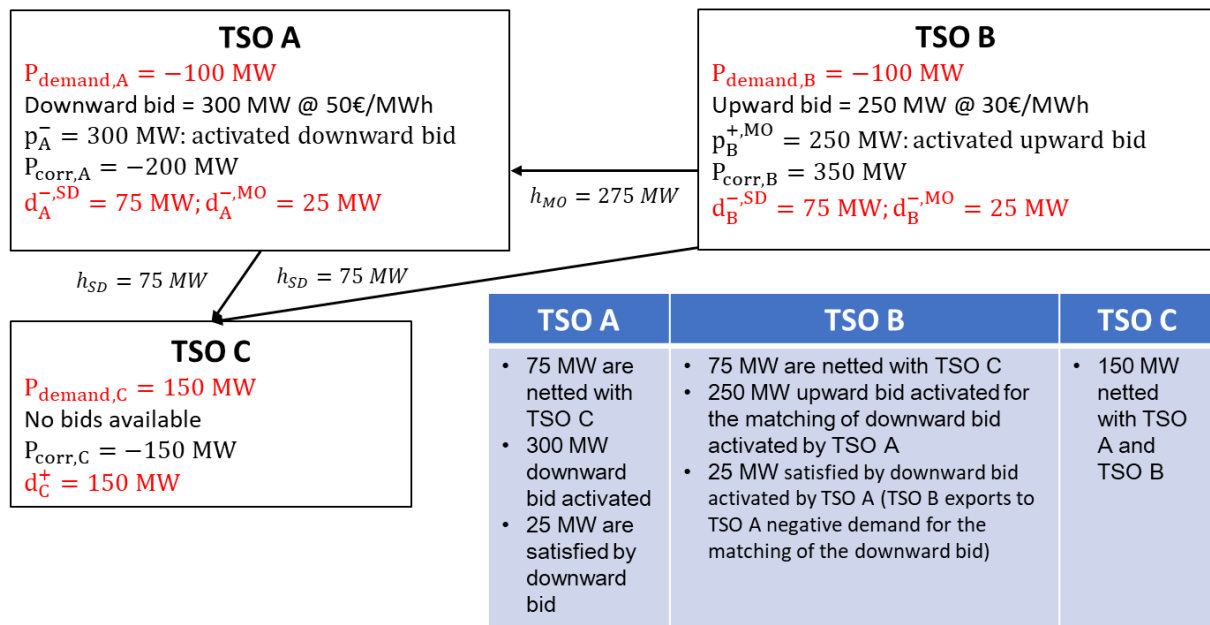
Figure 5: Example of satisfaction of demand and activation of offers with full allowance of counter-activations. In the picture, P_{demand} is the demand (inelastic part) of each LFC area, p^- is the activated downward bid, p^{+,MO} the activated upward bid to match negative offers, d^{-SD} and d^{-MO} are negative demands (inelastic part) satisfied by netting of offers, respectively. d^+ is the satisfied positive demand (inelastic part) and P_{corr} is the correction value.
