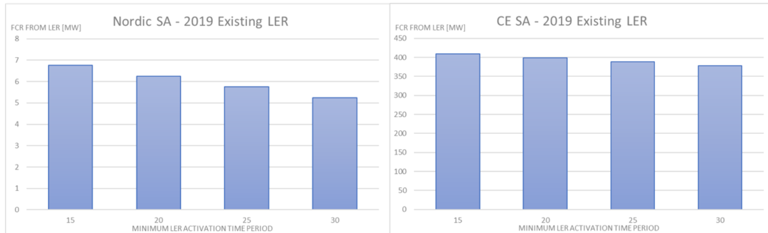
Effect of different minimum activation Time Period on electrochemical storage in both SAs
