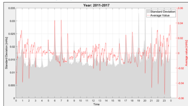
2011-2017 CE Daily frequency deviation
